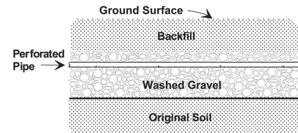
Image: Example layers in the drainfield.
