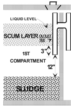
Image: Layers in the tank
