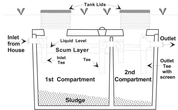
Image: Inside the septic tank.
