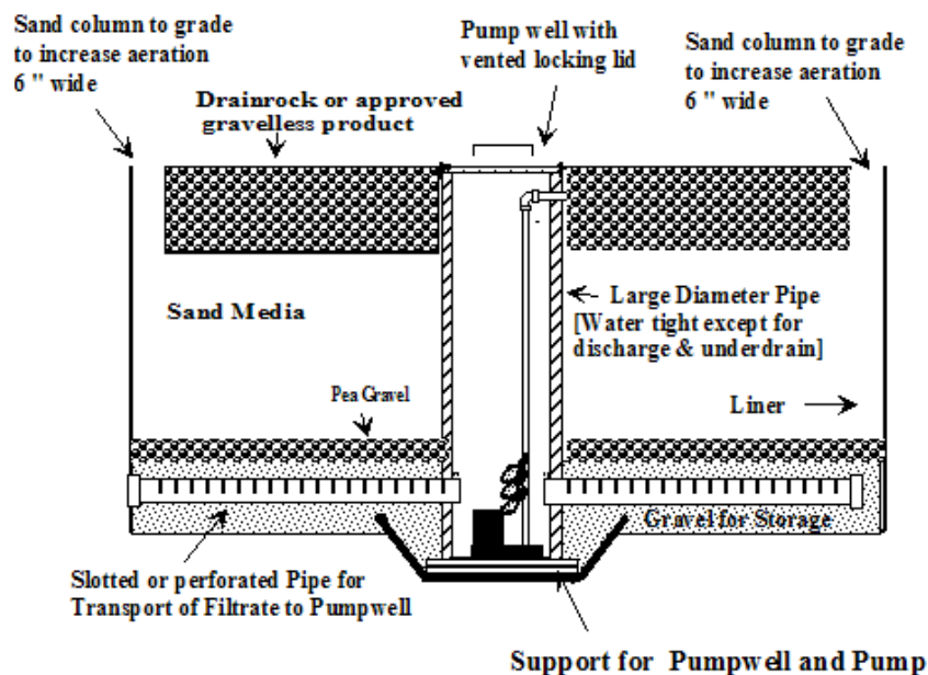
Figure 6 - Examples of Sand Filter Construction Methods to Increase Aeration
