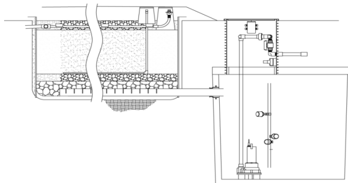
Figure 4 - Example: Gravity Discharge Underdrain to External Pump Tank, Cross Section
