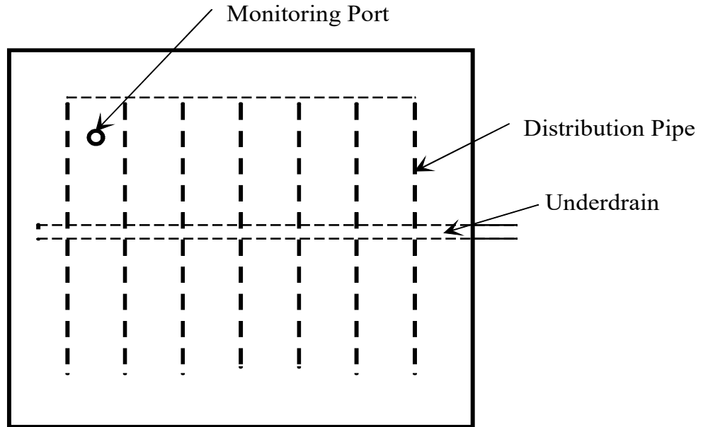
Figure 3 - Typical Intermittent Sand Filter, Top View
