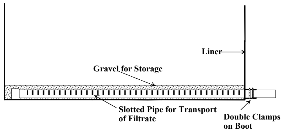
Figure 7 - Typical Cross-section of a Gravity Discharge Underdrain
