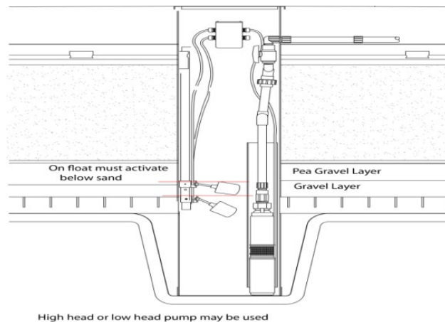
Figure 5 - Example: Internal Pump Basin Assembly (w/ Float Setting Detail)
