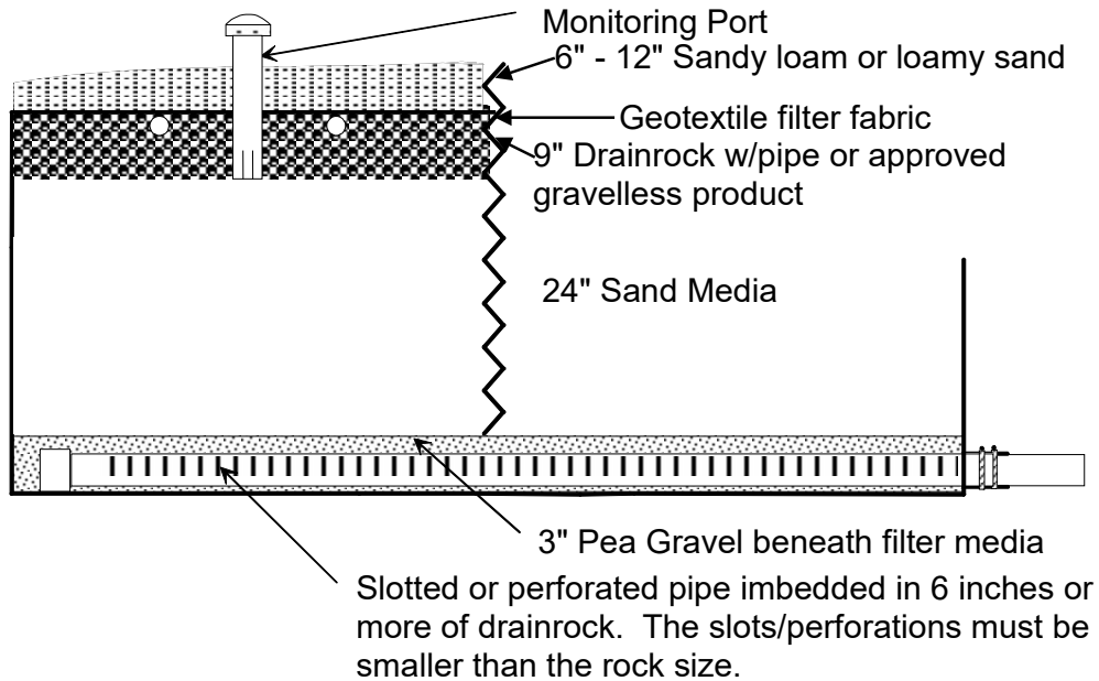
Figure 2 - Typical Intermittent Sand Filter, Cross Section
