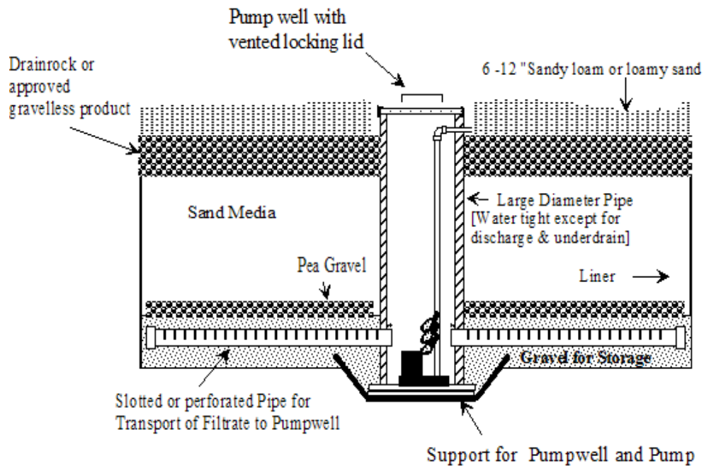
Figure 8 - Typical Cross-section of an Pump Discharge Underdrain
