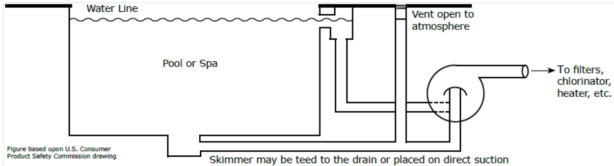
Figure 1. Suction Limiting Vent System
