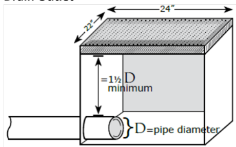
Figure 4. Example 1 of Unblockable Drain Outlet
