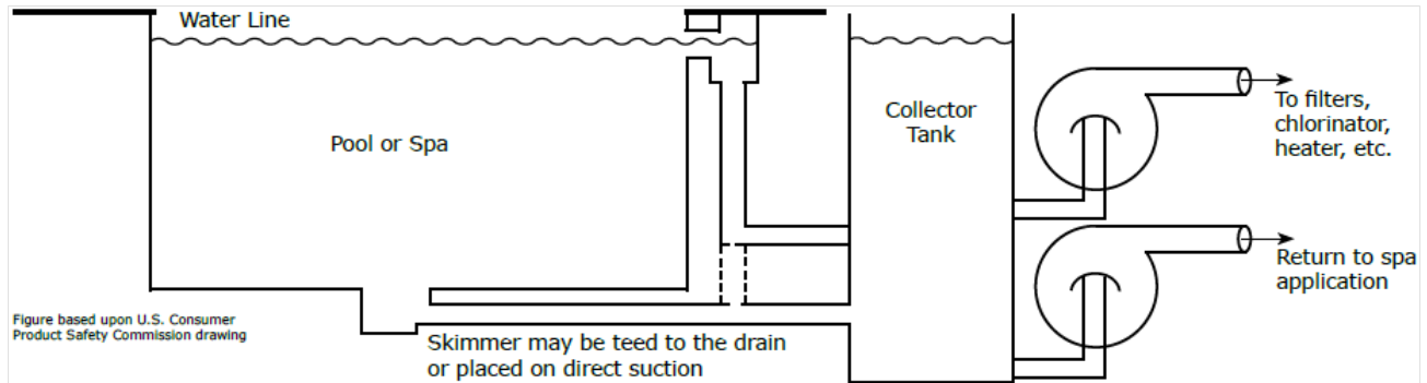
Figure 2. Gravity Drainage System
