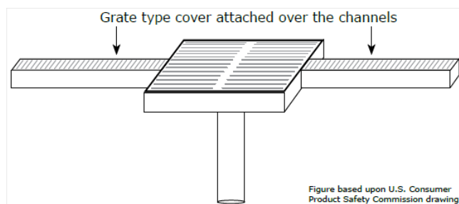
Figure 5. Example 2 of Unblockable Drain Outlet
