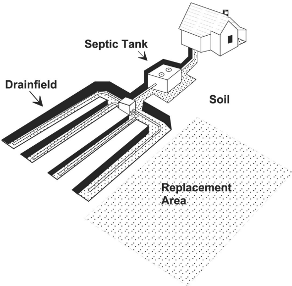
Image: Diagram of a basic septic system
