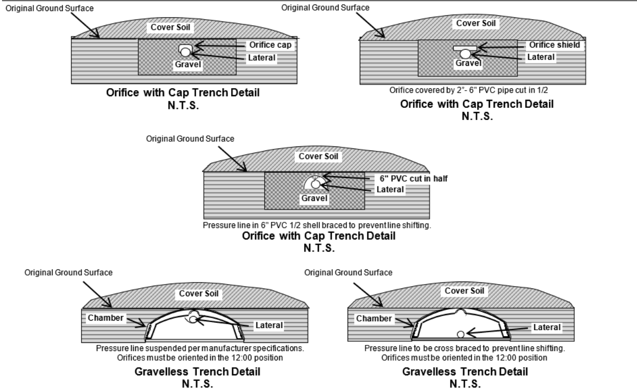
Figure 7. Orifice Caps and Shields
