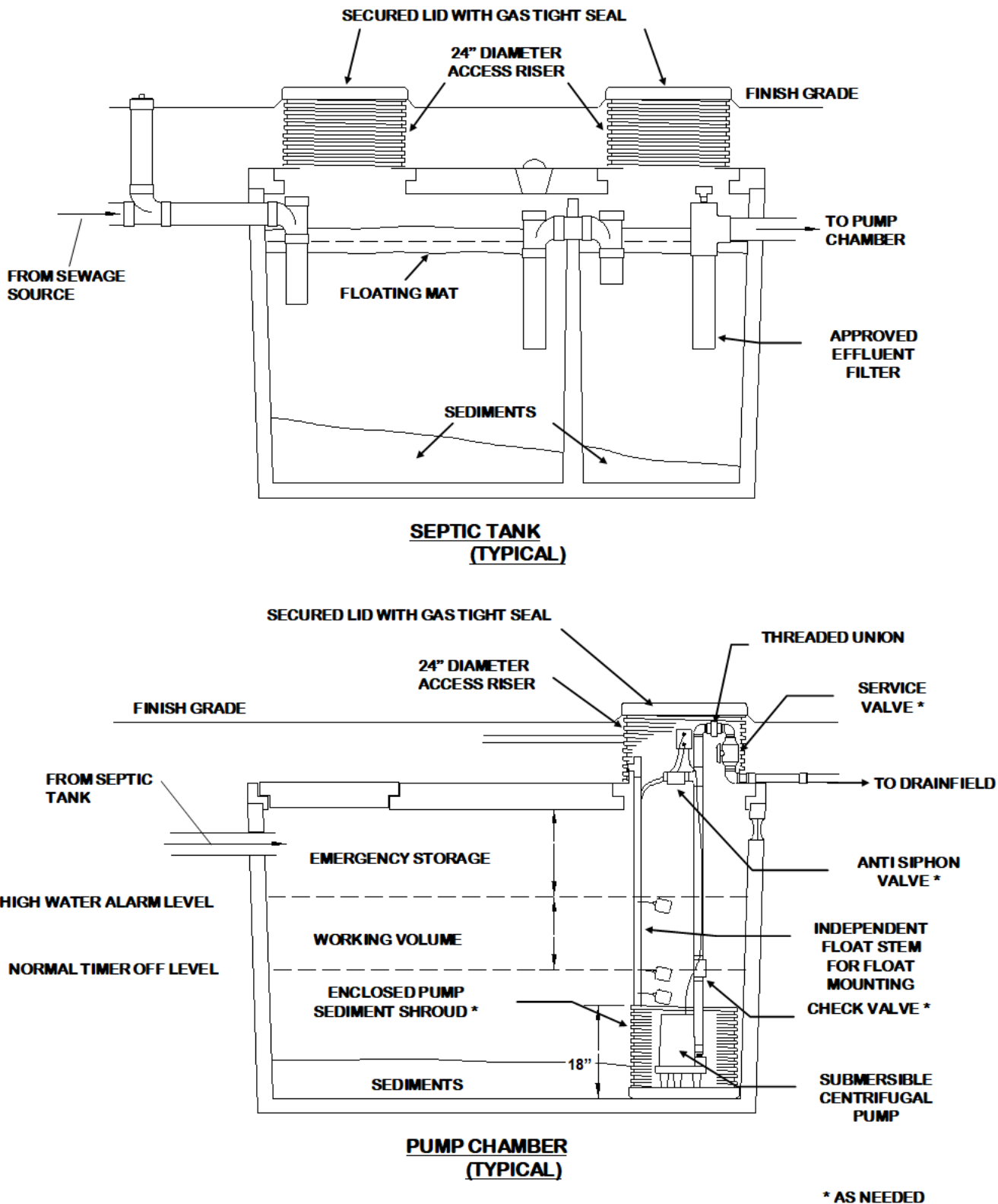
Figure 2. Typical Septic Tank and Pump Chamber
