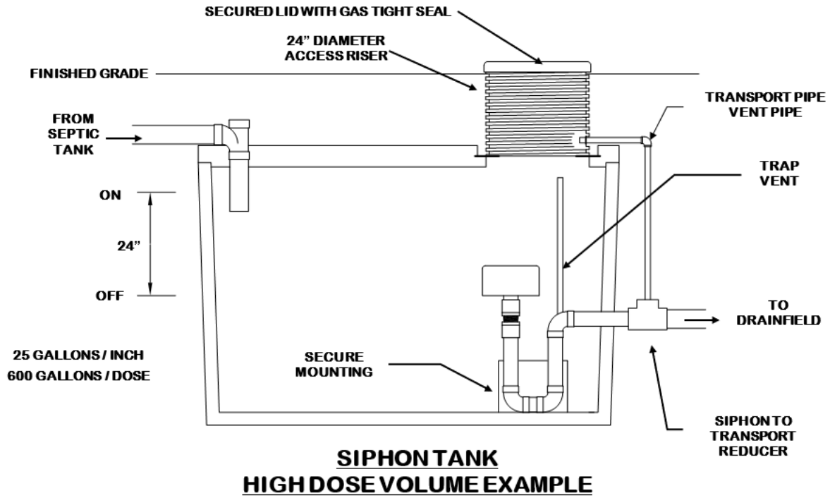
Figure 10. Siphon Tank High/Low Dose Volume Examples
