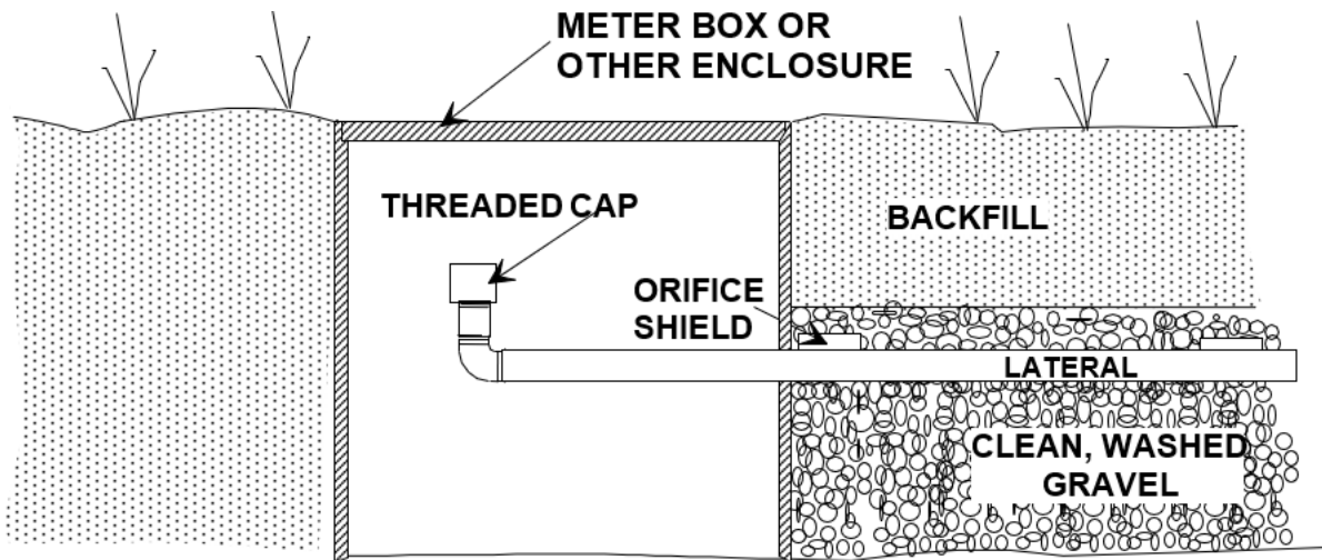
Figure 8A. Cleanout and Monitoring Port
