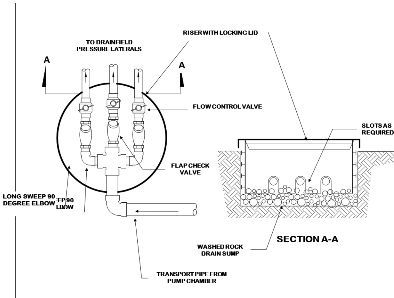
Figure 6A. Drainfield Control Box (Sloping Ground, Manifold Below Laterals)
