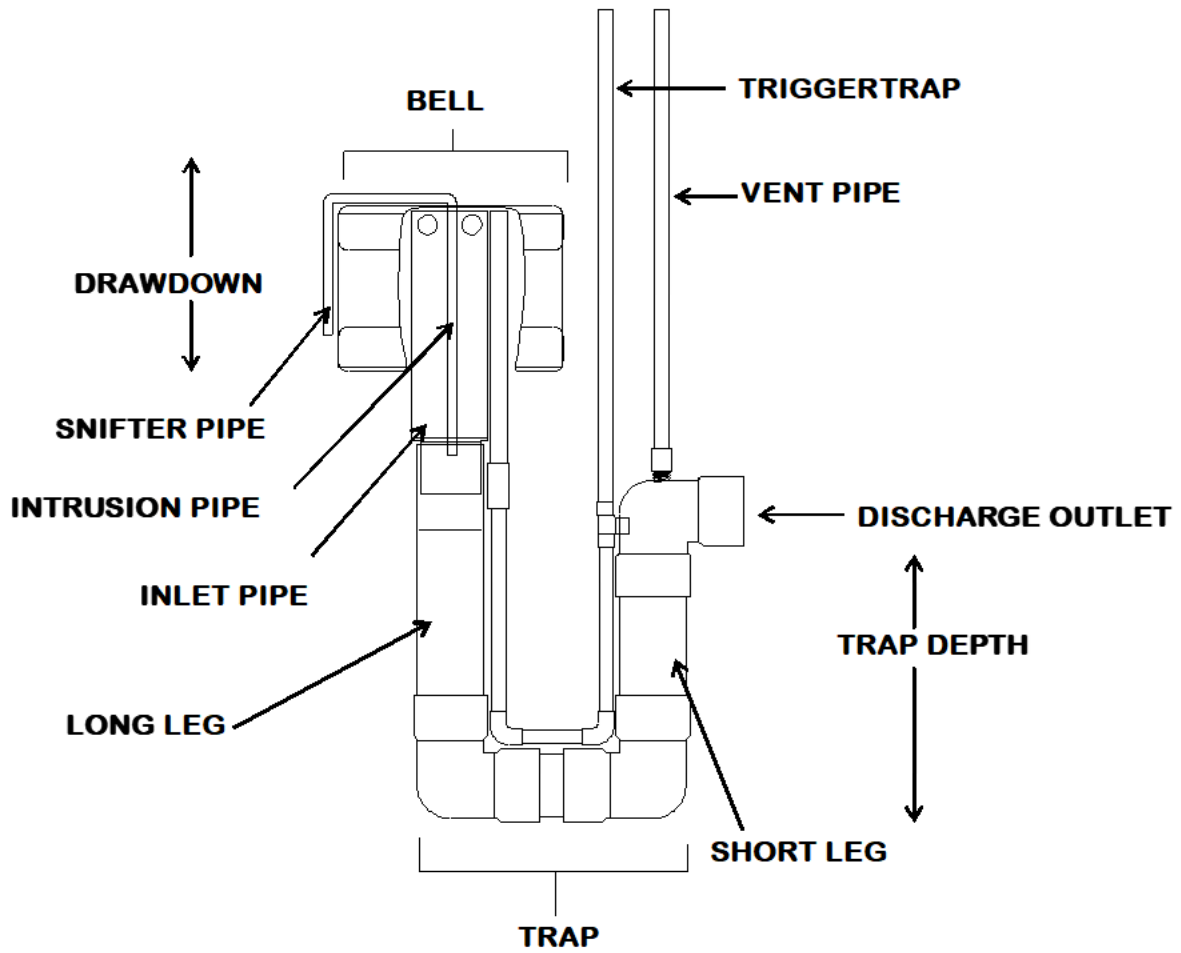
Figure 9. Example of Siphon
